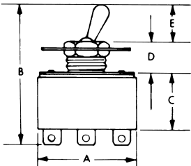
Mounting Hole: 0.500" Bushing .472 OD
