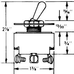
Mounting Hole: 0.500"
