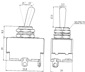
Mounting Hole: 0.500"
